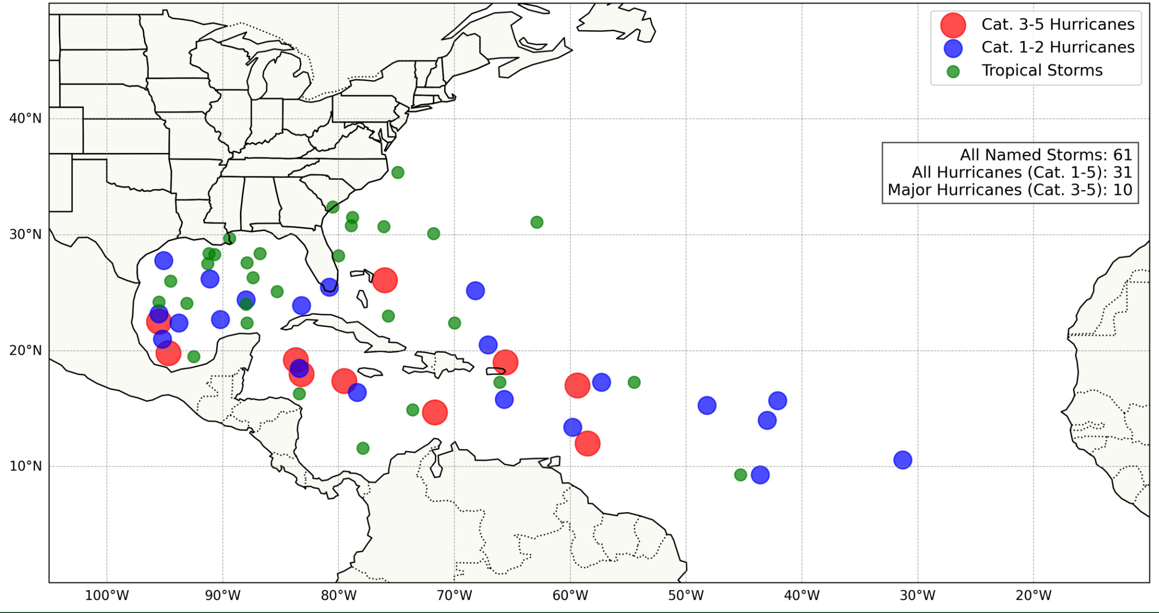
CONUS Landfall Formation Locations during 15 Coldest La Niña Years Since 1950 (ASO RONI \leq -0.76 )
