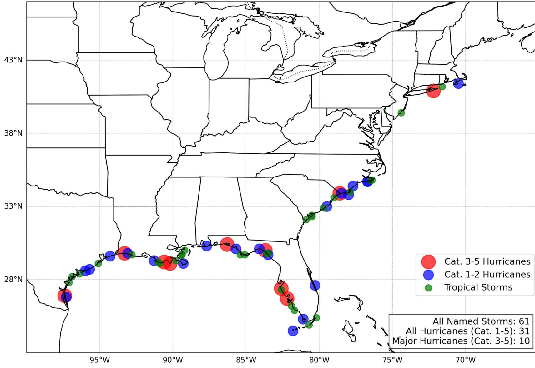
CONUS Landfalls during 15 Coldest La Niña Years Since 1950 (ASO RONI \leq -0.76 )
